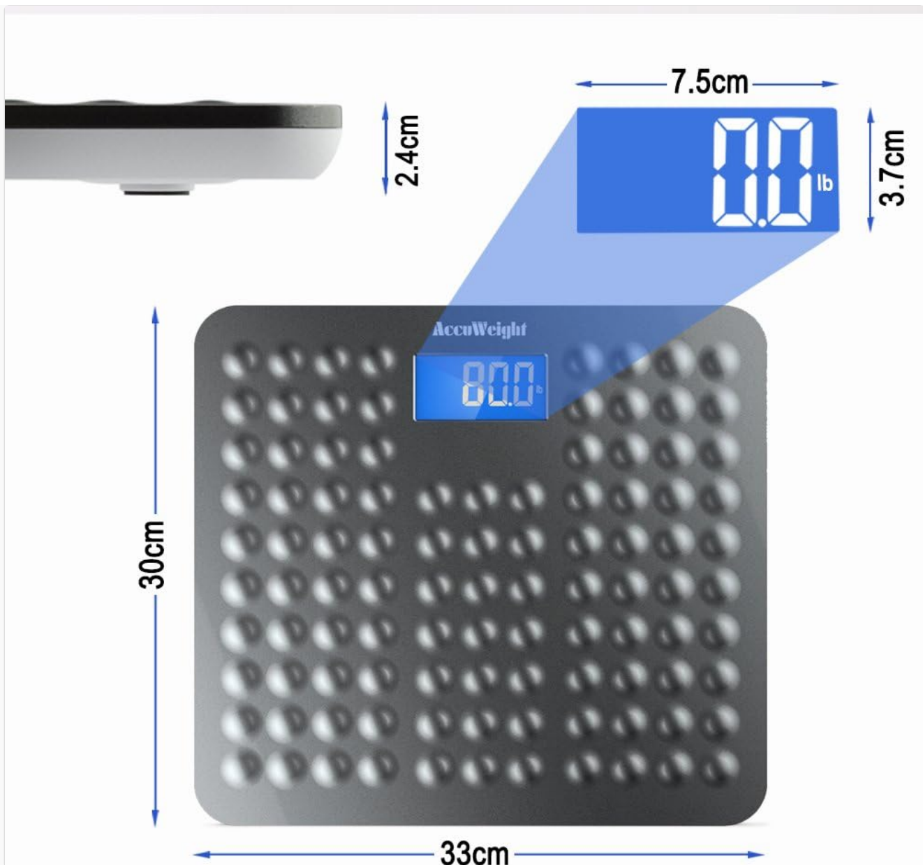
Image: Technical drawing of the Accuweight scale, illustrating its dimensions: 33 cm (length), 30 cm (width), and 2.4 cm (height), along with the display size.
