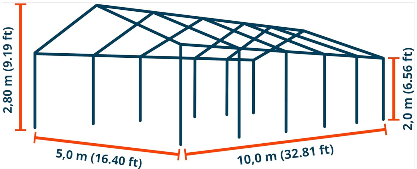
Image: Dimensional diagram of the storage tent (10m L x 5m W x 2.9m H).
