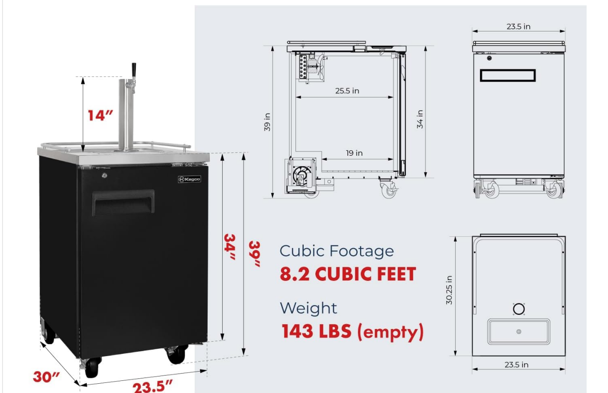
Figure 8: Dimensional drawing of the Kegco XCK-1B Kegerator.
