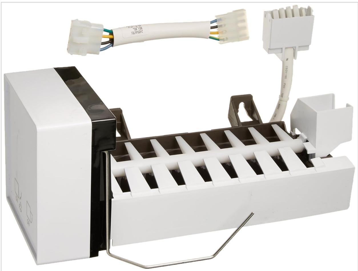
Figure 1: FRIGIDAIRE 5303918277 Ice Maker Replacement unit, showing the main body, ice mold, and electrical connector.
