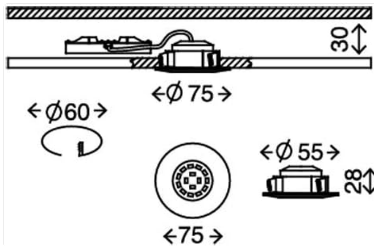
Image 5.1: Installation Dimensions and Diagram
