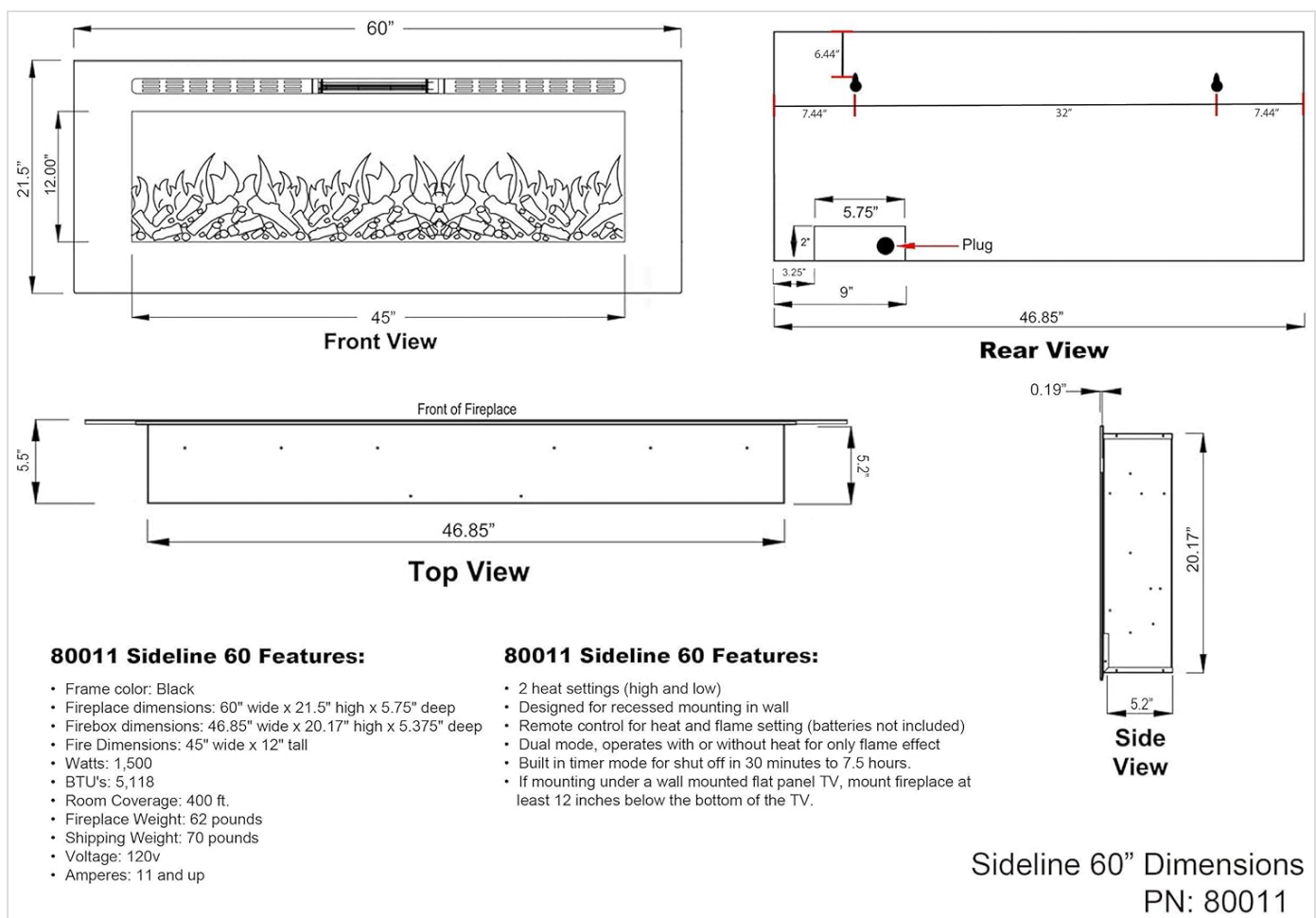
Figure 3.1: Detailed dimensions for the Touchstone Sideline 60-inch electric fireplace, including rough opening requirements for recessed installation.
