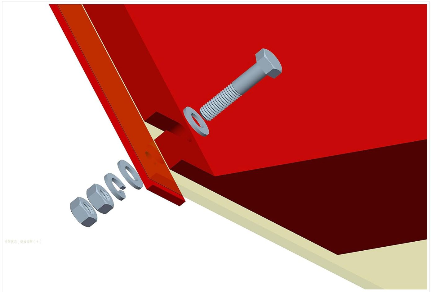
Figure 3: Illustration of the bolt, washer, and nut assembly for securing the pad to the compactor.
