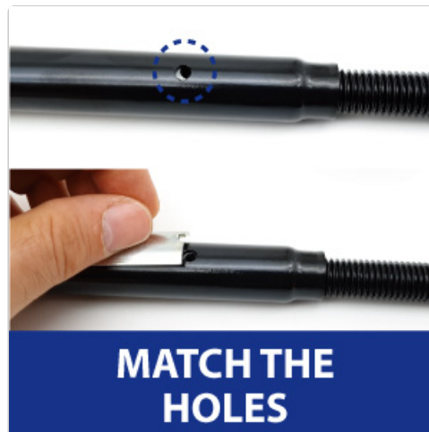
Image: Demonstrates lowering the steering wheel to its lowest position for proper lock installation.
