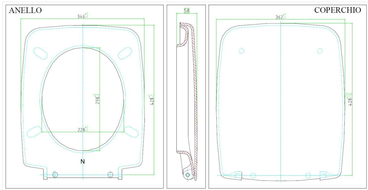
Image: Technical drawing illustrating the dimensions of the Cantica toilet seat and lid, including hinge spacing.
