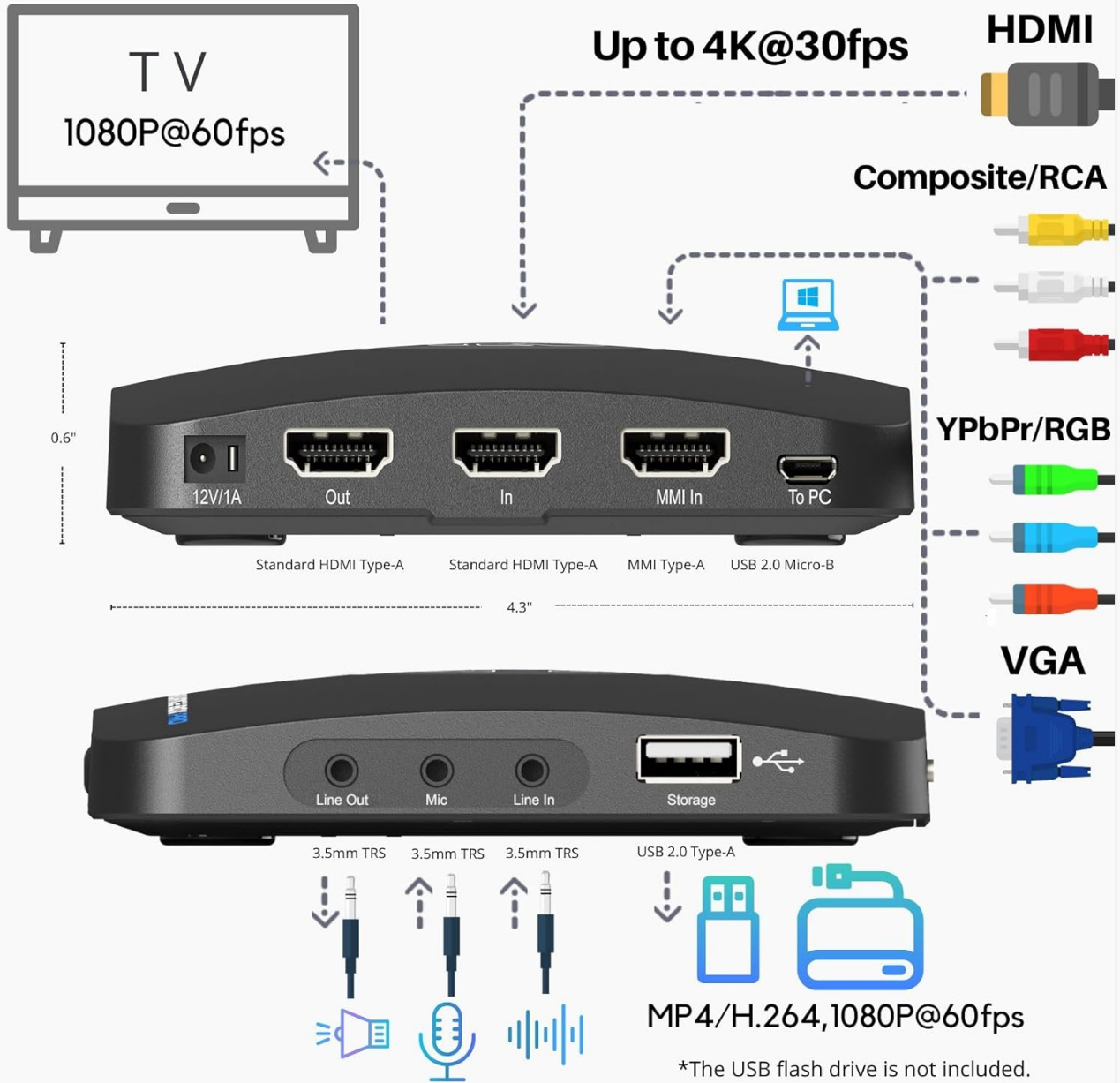
Image 4.1: Detailed diagram of ClonerAlliance Box Pro ports and connections.
