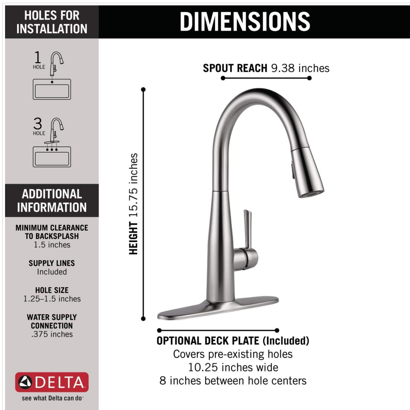
Figure 1: Faucet Dimensions and Hole Requirements. The faucet has a height of 15.75 inches and a spout reach of 9.38 inches. It is compatible with 1 or 3-hole installations, with an optional deck plate included.
