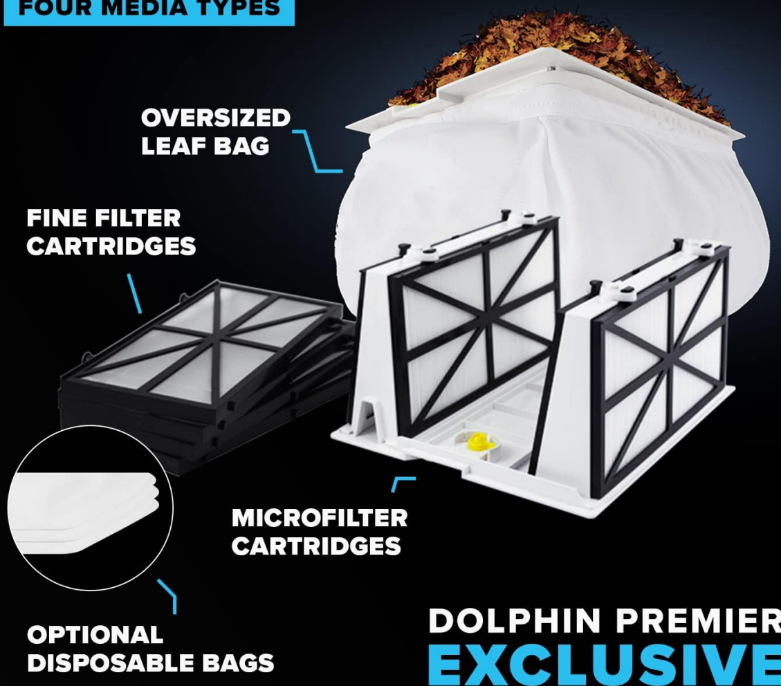
Image 4.1: The Dolphin Premier's multimedia filtration system, showcasing the oversized leaf bag, fine filter cartridges, and microfilter cartridges.
