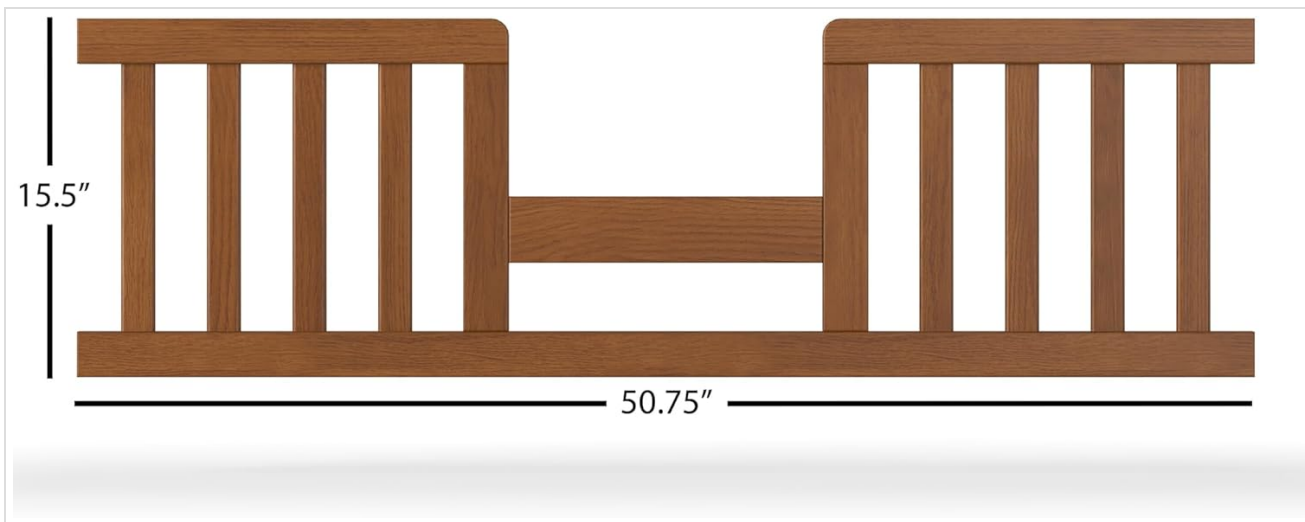
Image: The Child Craft Toddler Guard Rail with key dimensions indicated.
