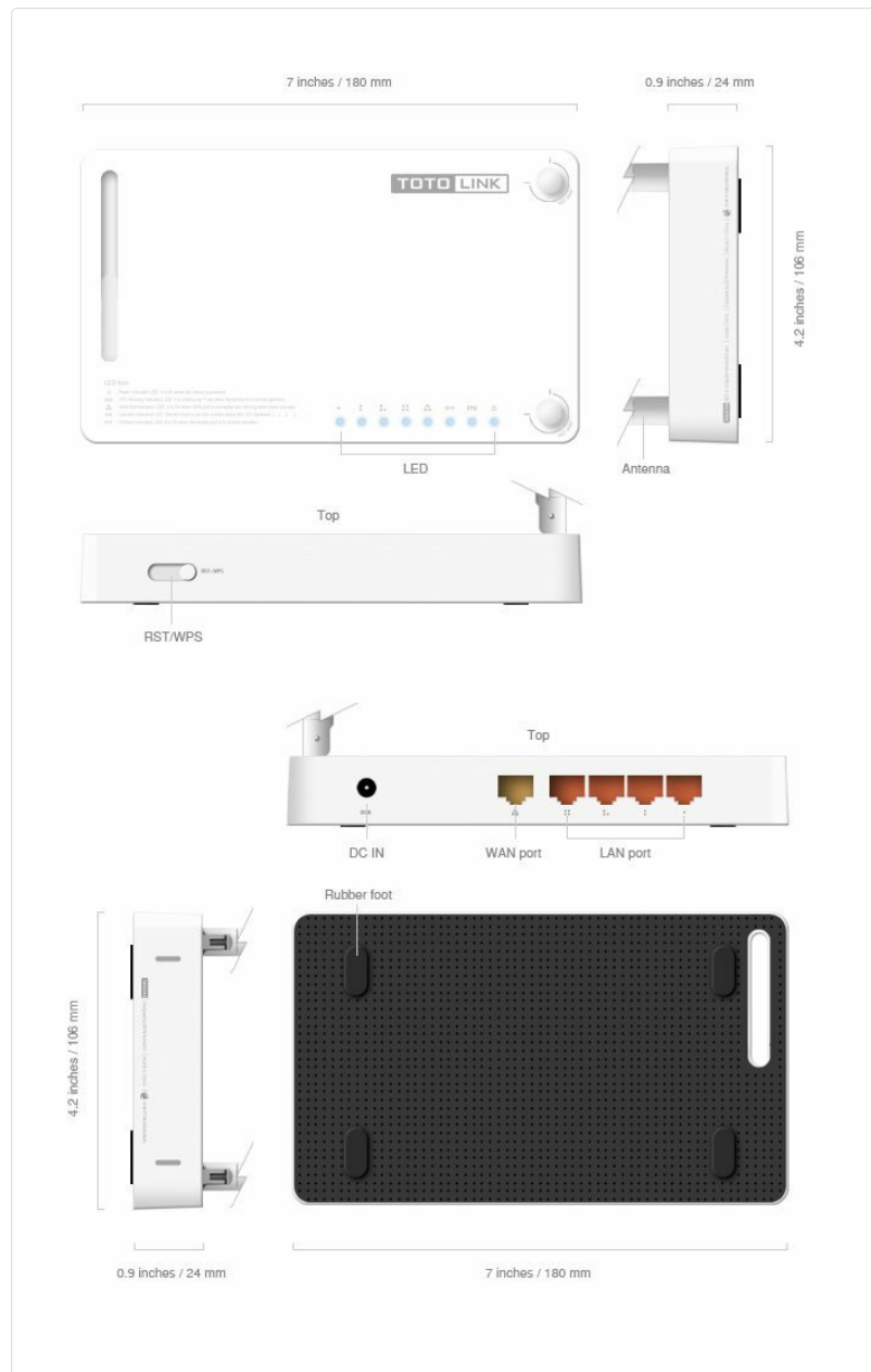
Figure 4.2: Detailed diagram of the TOTOLINK N300RH, illustrating its top, side, and bottom views with dimensions and port labels. Key components include LED indicators, RST/WPS button, DC IN port, WAN port, LAN ports, and rubber feet.
