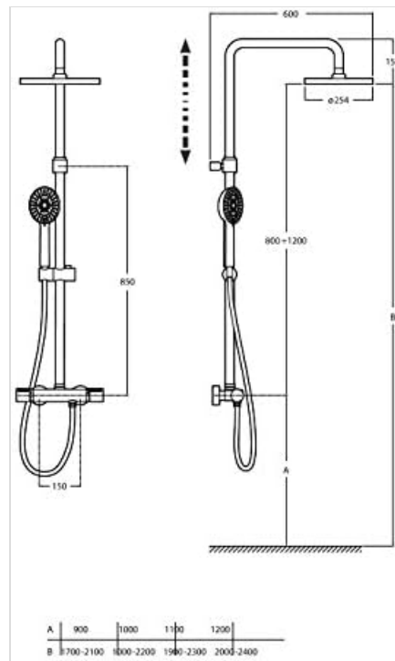
Image 4.1: Technical diagram illustrating the dimensions and installation points for the Roca Victoria A5A9780C00 Shower Column, including adjustable height ranges.
