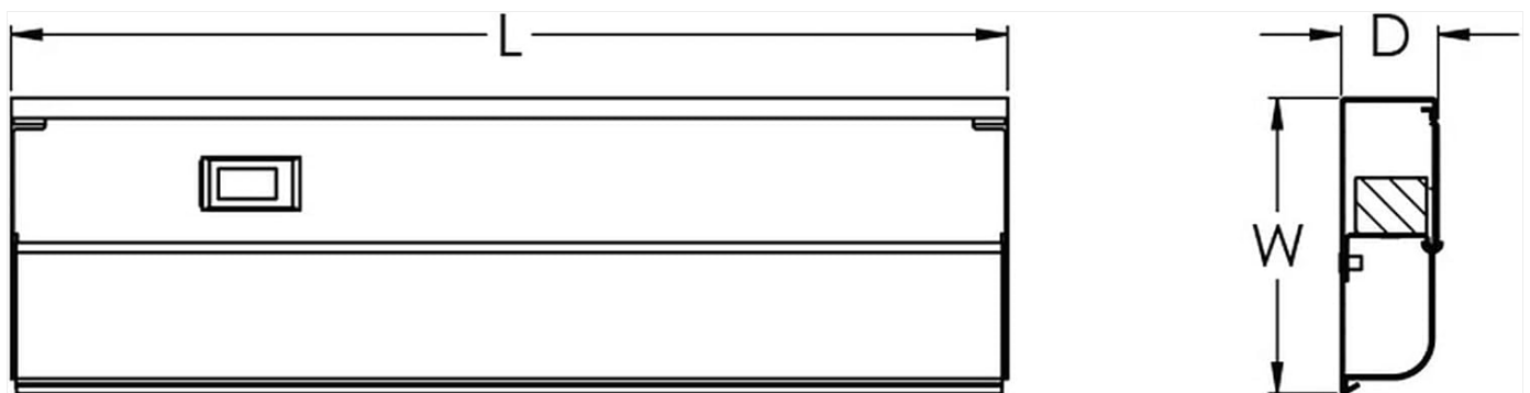
Image 4.1: Dimensional diagram of the AFX Under Cabinet Light, showing length (L), width (W), and depth (D) for installation planning.
