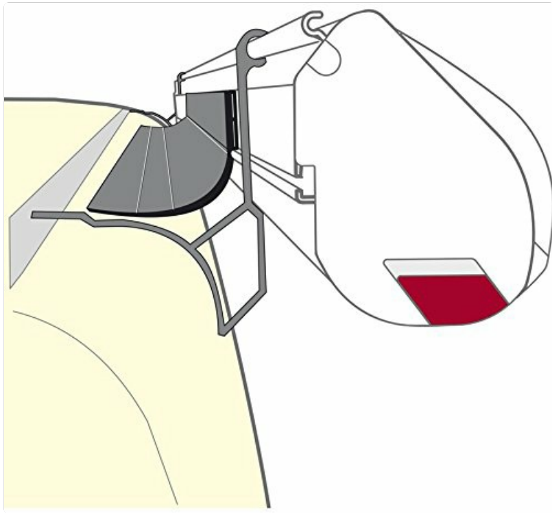
Image 1: Fiamma 98655-947 Rain Guard Van Seal Kit. This image shows the black rubber seal kit, which is used to prevent water from entering the gap between a campervan's awning and its body.
