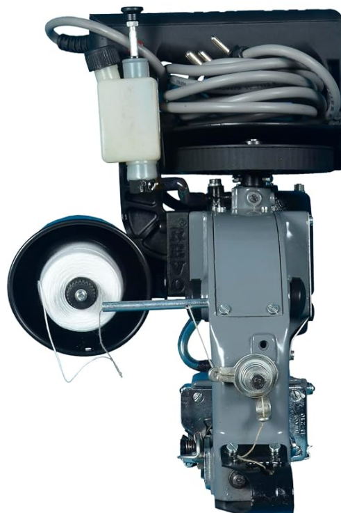
Figure 3.3: Side view of the machine, detailing the thread path and tension adjustments.
