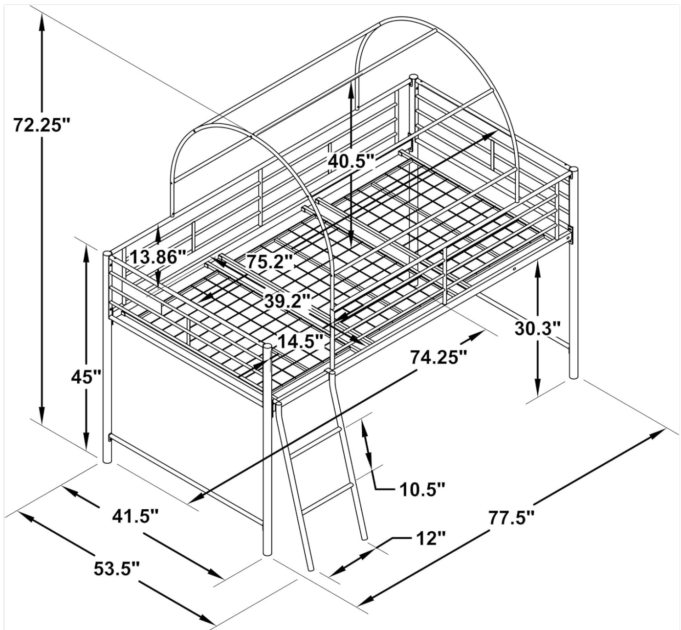
Image 7.1: Detailed dimensional diagram illustrating the length, width, and height measurements of the loft bed frame.
