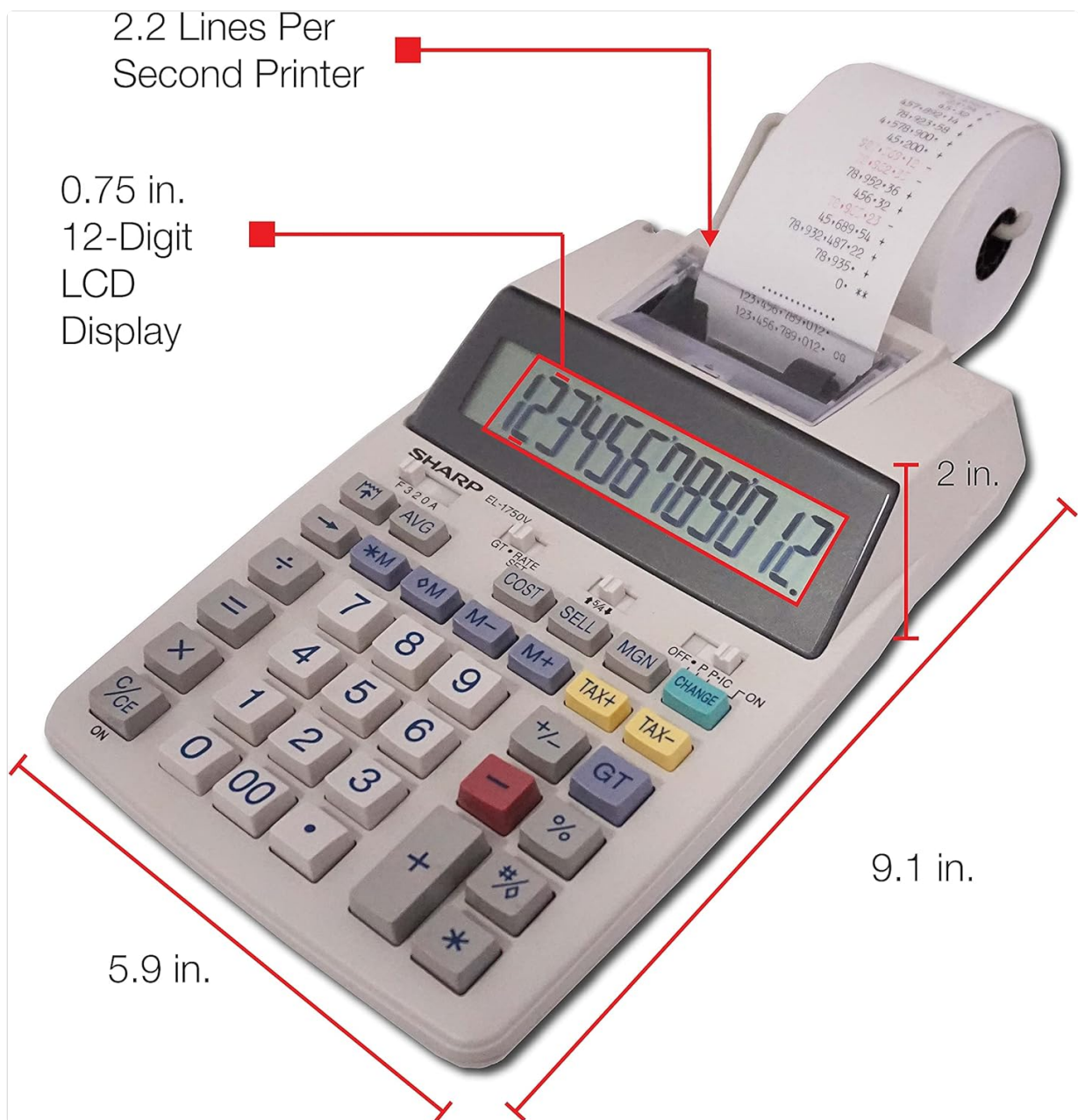
Figure 4: Dimensions of the Sharp EL1750V calculator, showing a width of 5.9 inches, depth of 9.1 inches, and height of 2 inches, with a 0.75 inch 12-digit LCD display.
