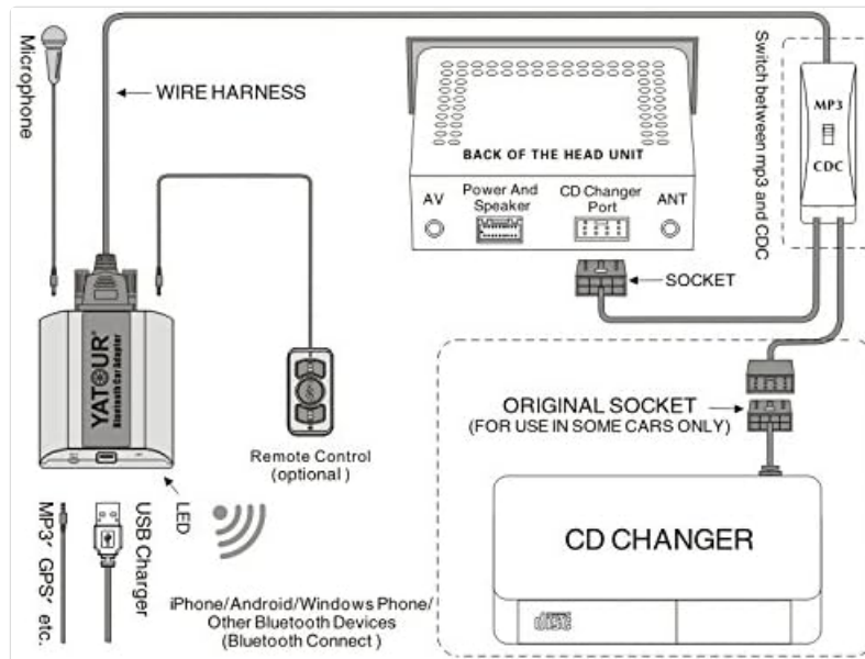
Image: Detailed wiring diagram illustrating how to connect the Yatour Bluetooth Car Adapter to the car's head unit, including connections for the microphone and optional remote control.
