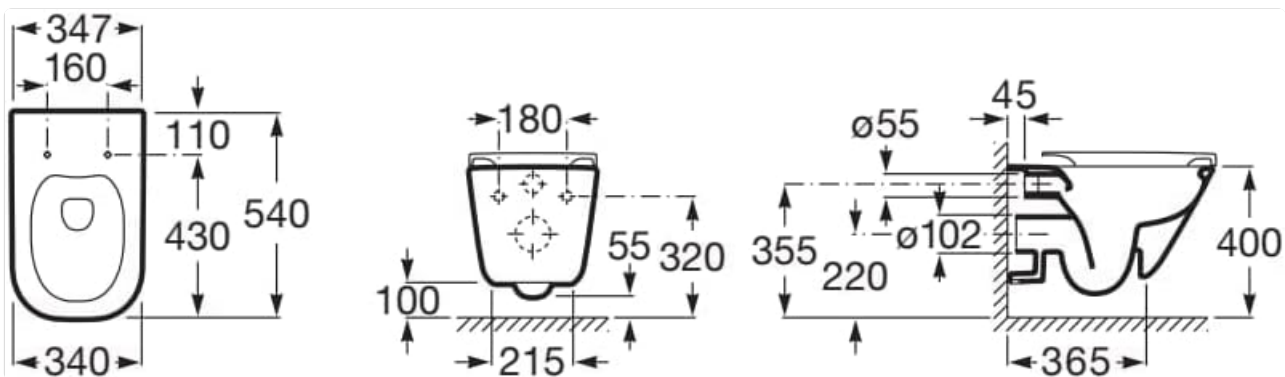
Figure 2: Technical drawing showing the dimensions and installation points for the Roca Clean Rim SQUARE toilet pan. This diagram provides critical measurements for rough-in and final placement, including top, front, and side views with all relevant dimensions in millimeters.
