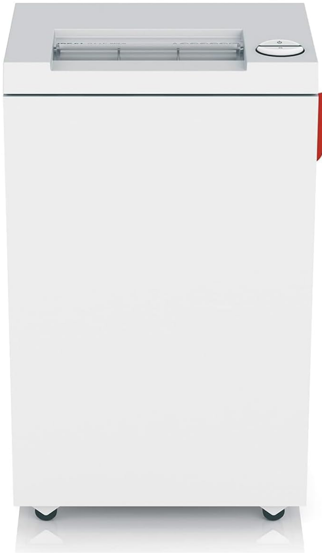
Figure 4: Visual representation of the shredder's capacity. The IDEAL 2445 can shred up to 13 sheets of paper at once and has a 35-liter (9-gallon) waste bin capacity.
