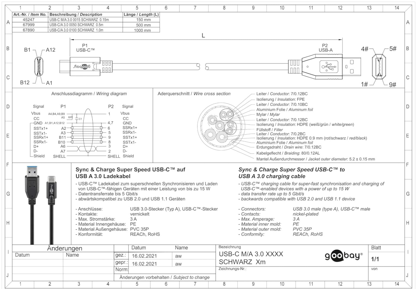
Image: A technical drawing of the Goobay USB-C to USB A 3.0 cable, showing detailed dimensions and internal wiring diagrams.
