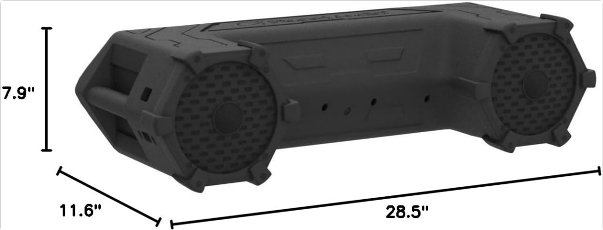
Image: A diagram showing the key dimensions of the Planet Audio PATV65 unit: 28.5 inches in width, 11.6 inches in depth, and 7.9 inches in height.
