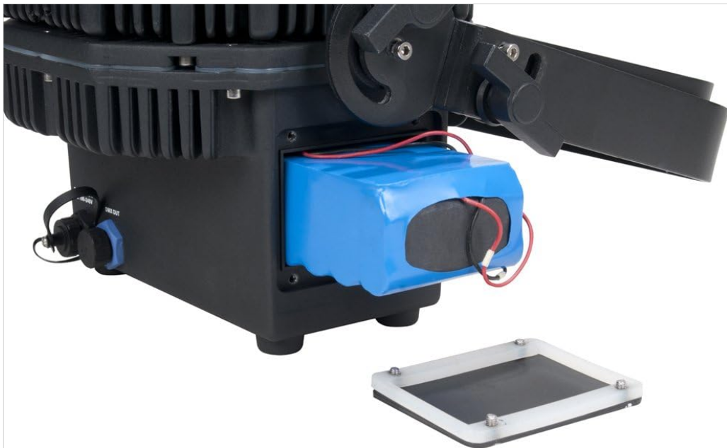
Image 4.2: Close-up view of the battery compartment on the ADJ WiFLY EXR HEX5 IP, showing the blue Lithium Ion battery pack partially exposed, indicating its removable nature for service.
