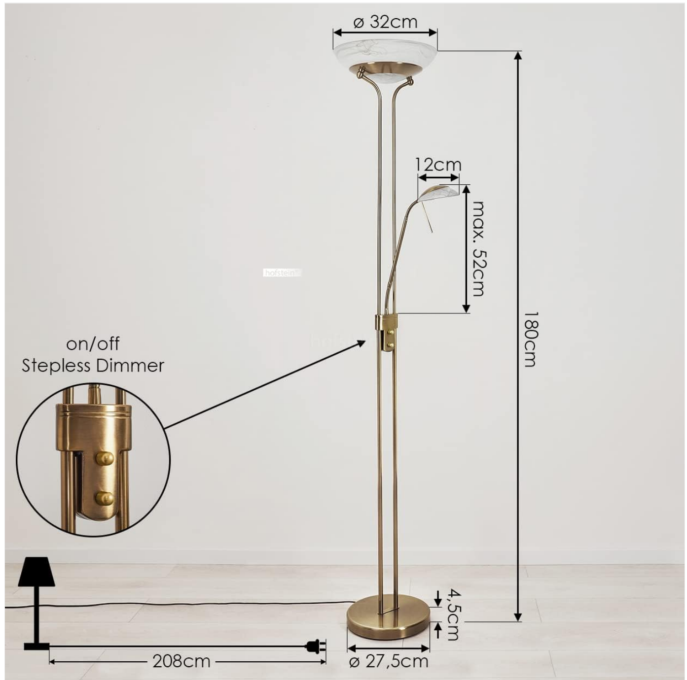
Image 4.1: Dimensional diagram and key components for assembly.
