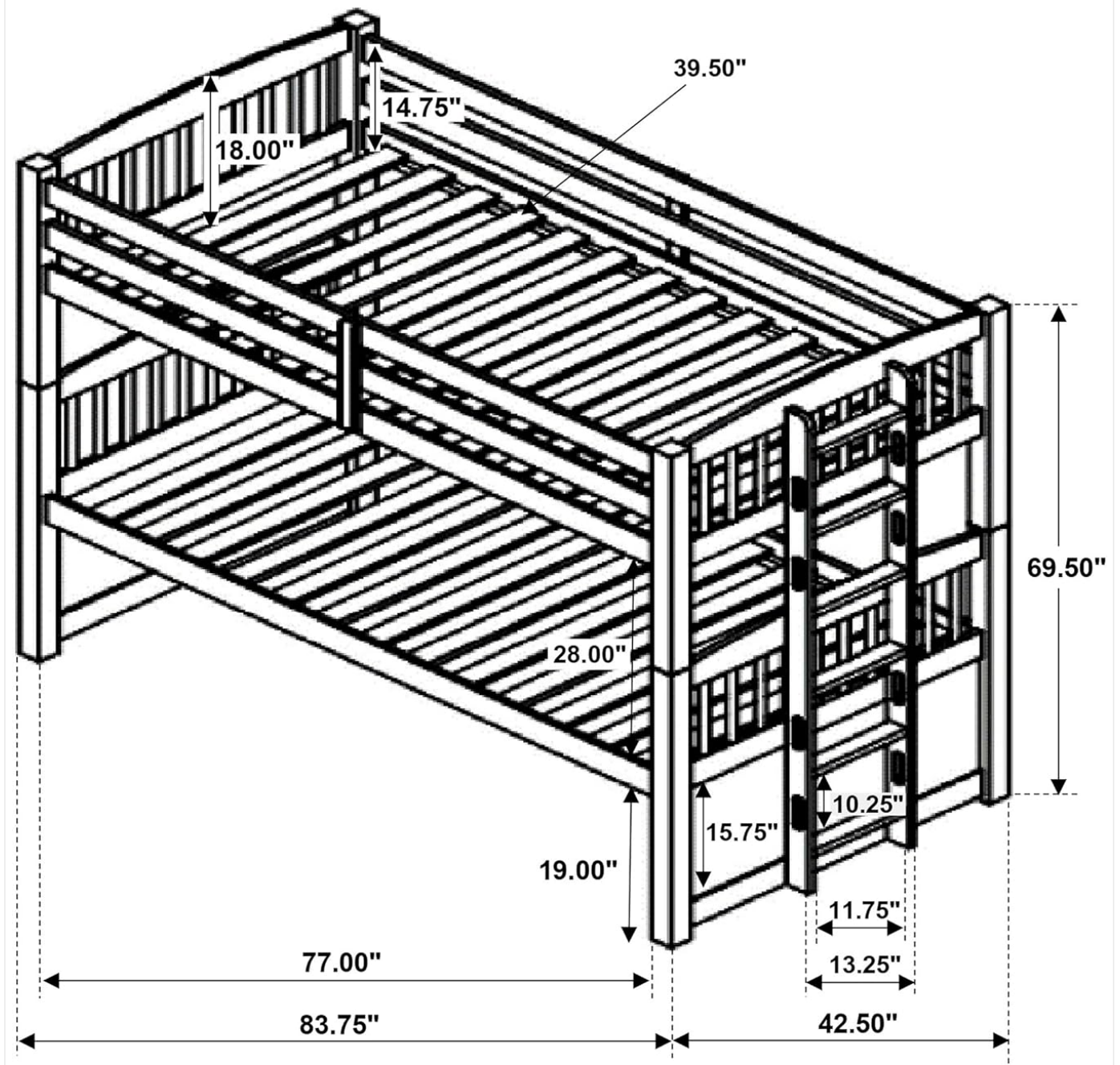
Figure 3: Dimensional drawing of the bunk bed, providing key measurements for space planning.
