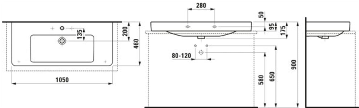
Figure 2: Technical drawing illustrating the dimensions and mounting points for the Laufen PRO S washbasin. All dimensions are in millimeters.
