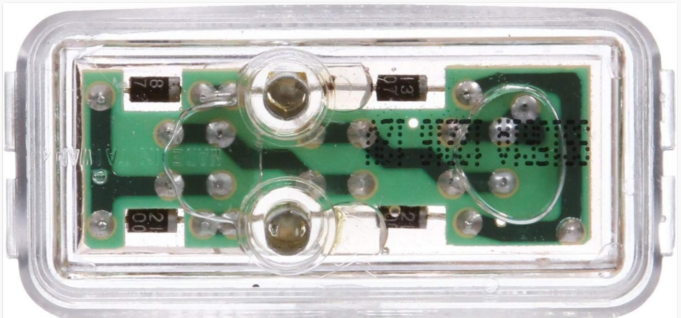
Figure 4.3: Rear view of the lamp, revealing the internal circuit board and wiring terminals.
