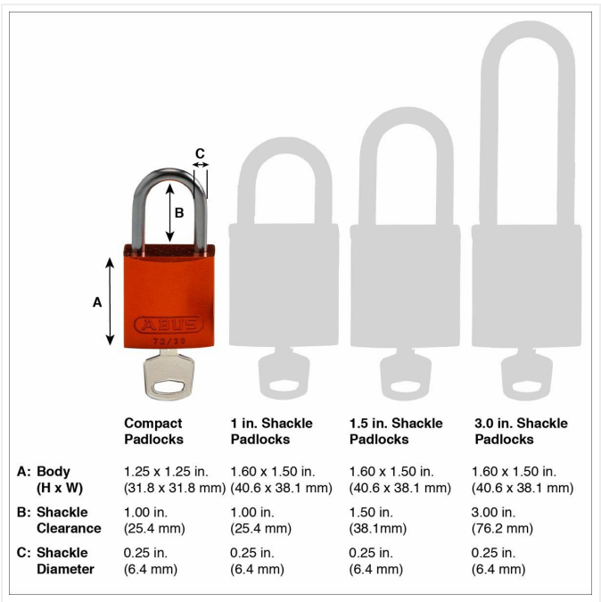
Image 2: Dimensional diagram illustrating key measurements for different padlock sizes. The Brady 133290 corresponds to the "Compact Padlocks" dimensions.
