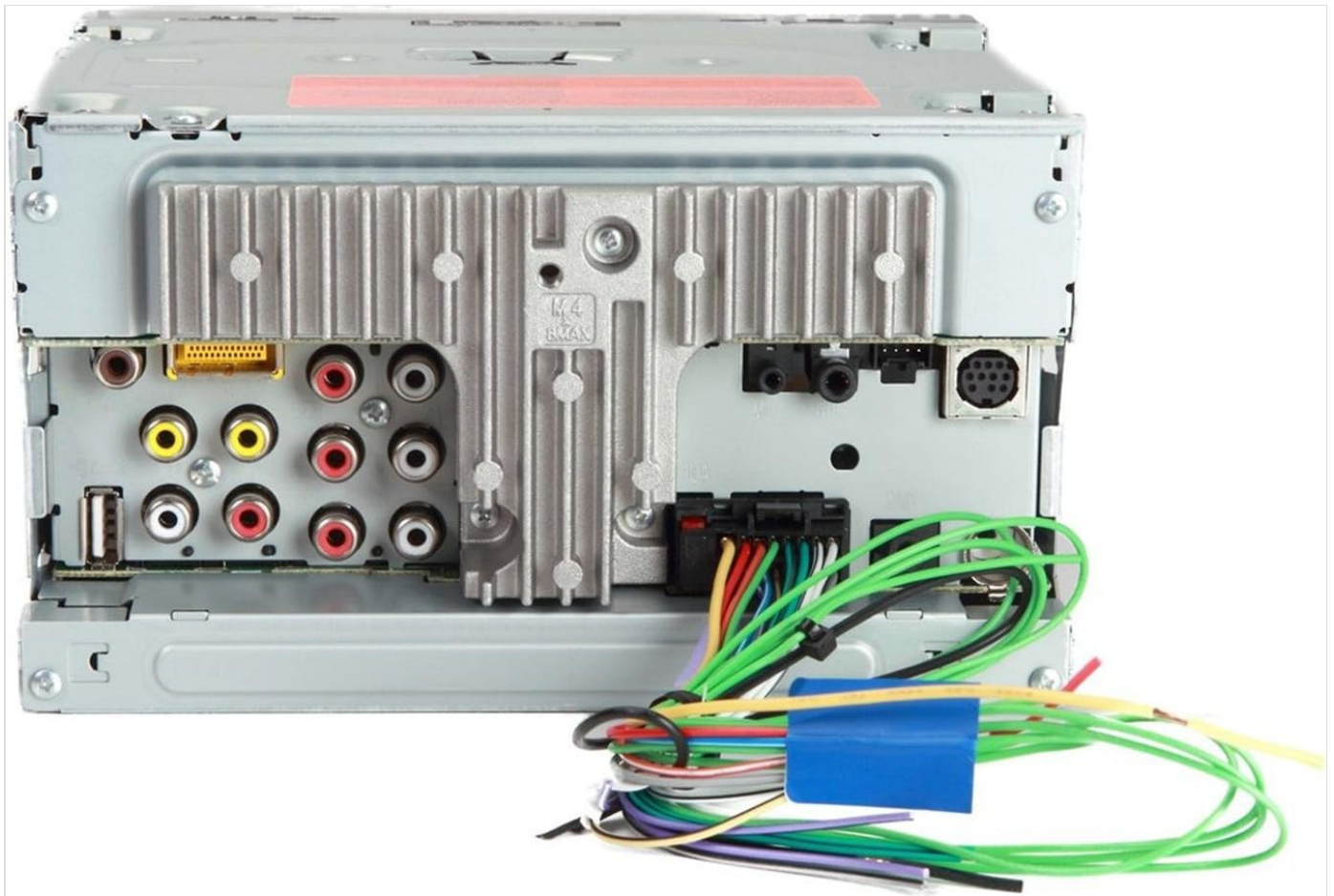
Figure 2.3: Rear view of the unit displaying various audio/video inputs, outputs, and power connections.
