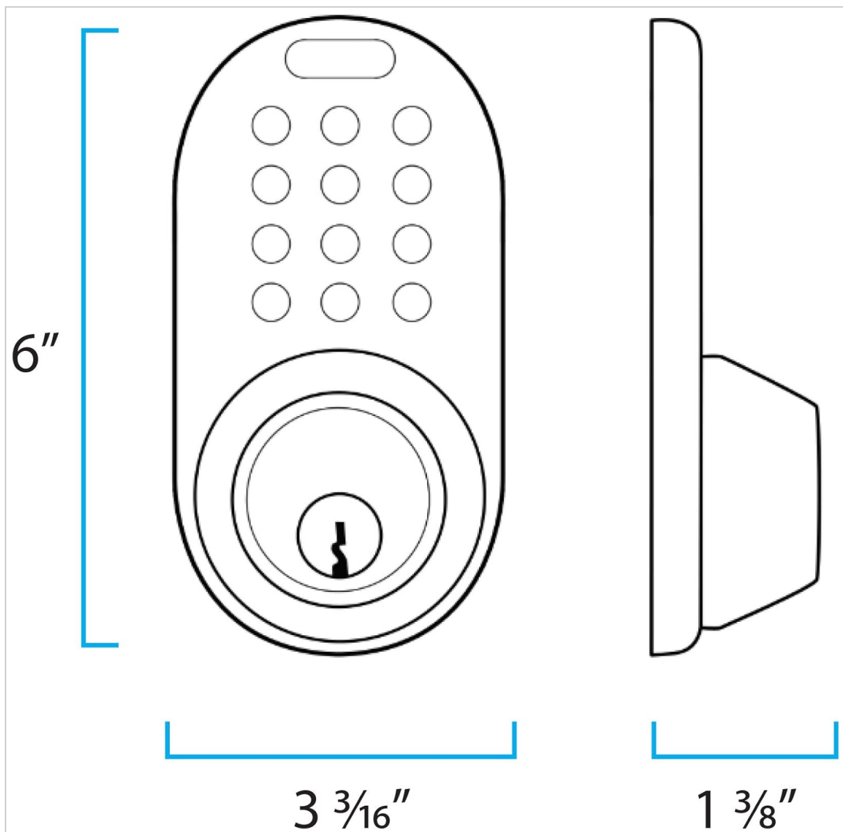
Figure 2: Side dimensions of the MiLocks DF-02AQ deadbolt, showing a depth of 1 3/8 inches for the front module and 1 3/4 inches for the back module.
