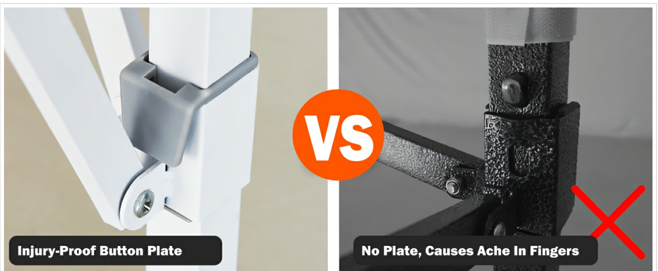
Figure 4.3: The improved injury-proof button plate design for safer operation.
