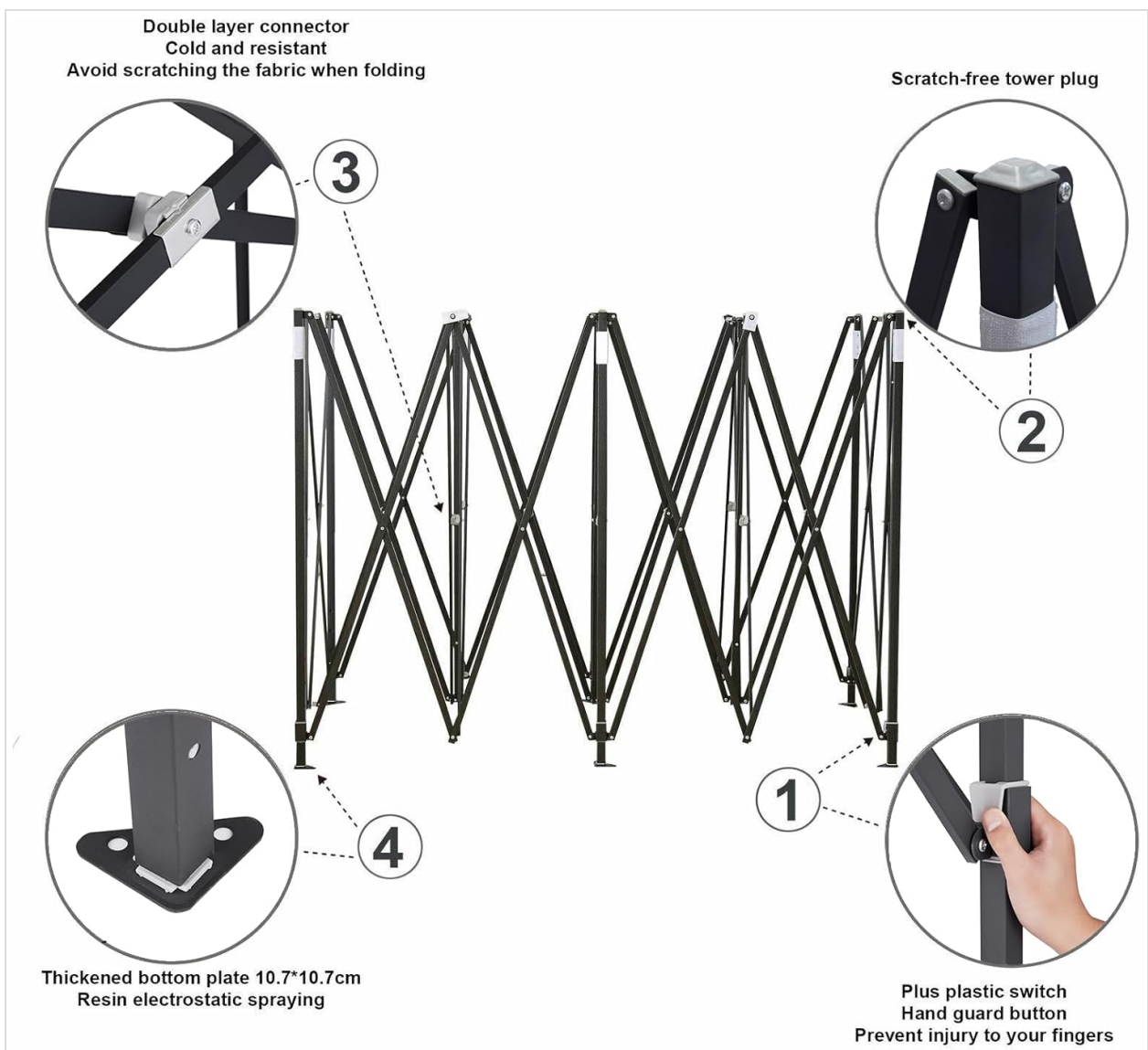
Figure 4.1: Key frame components including double layer connector, scratch-free tower plug, thickened bottom plate, and the
