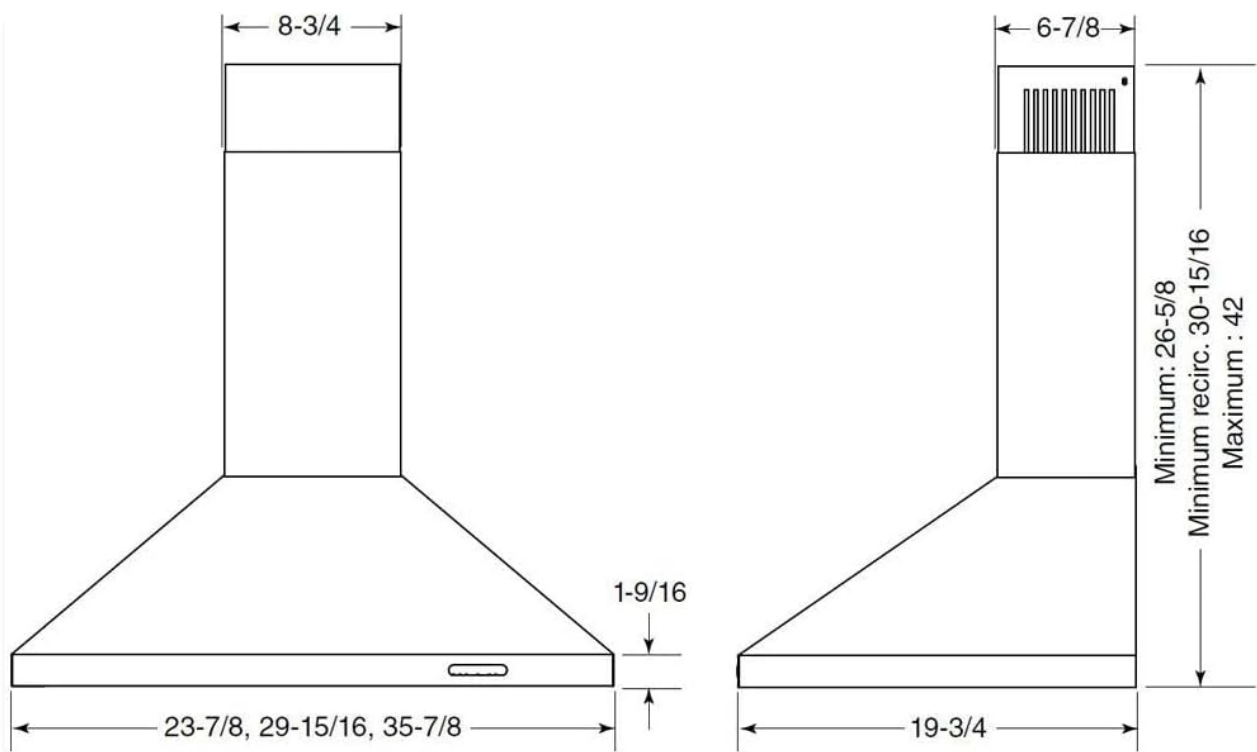
Image 2: Technical drawing illustrating the dimensions and mounting points of the range hood.
