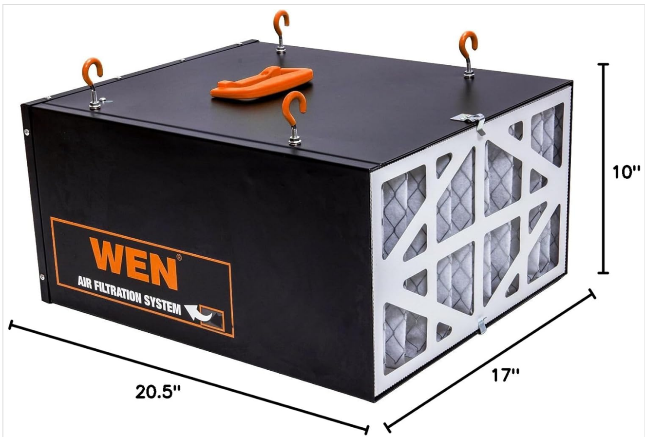
Image: Diagram showing the dimensions of the WEN 3410 Air Filtration System: 17 inches deep, 20.5 inches wide, and 10 inches high.
