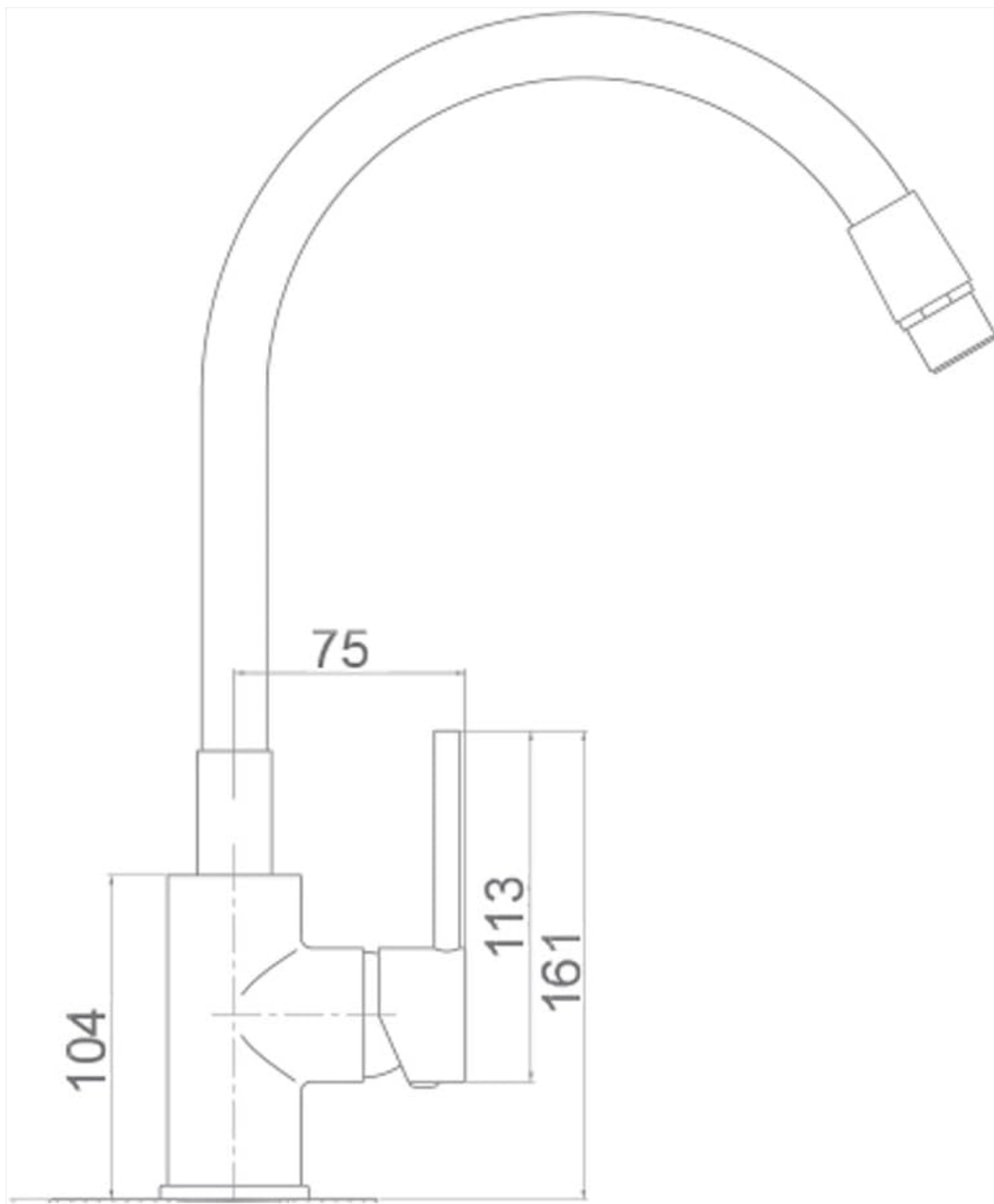
Image: Technical drawing illustrating the dimensions of the IMEX Verona GCE010 kitchen faucet.
