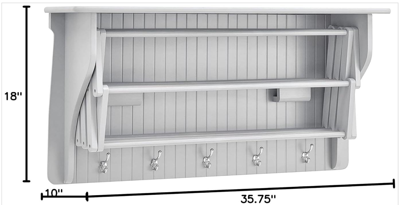
Figure 5: Product Dimensions
