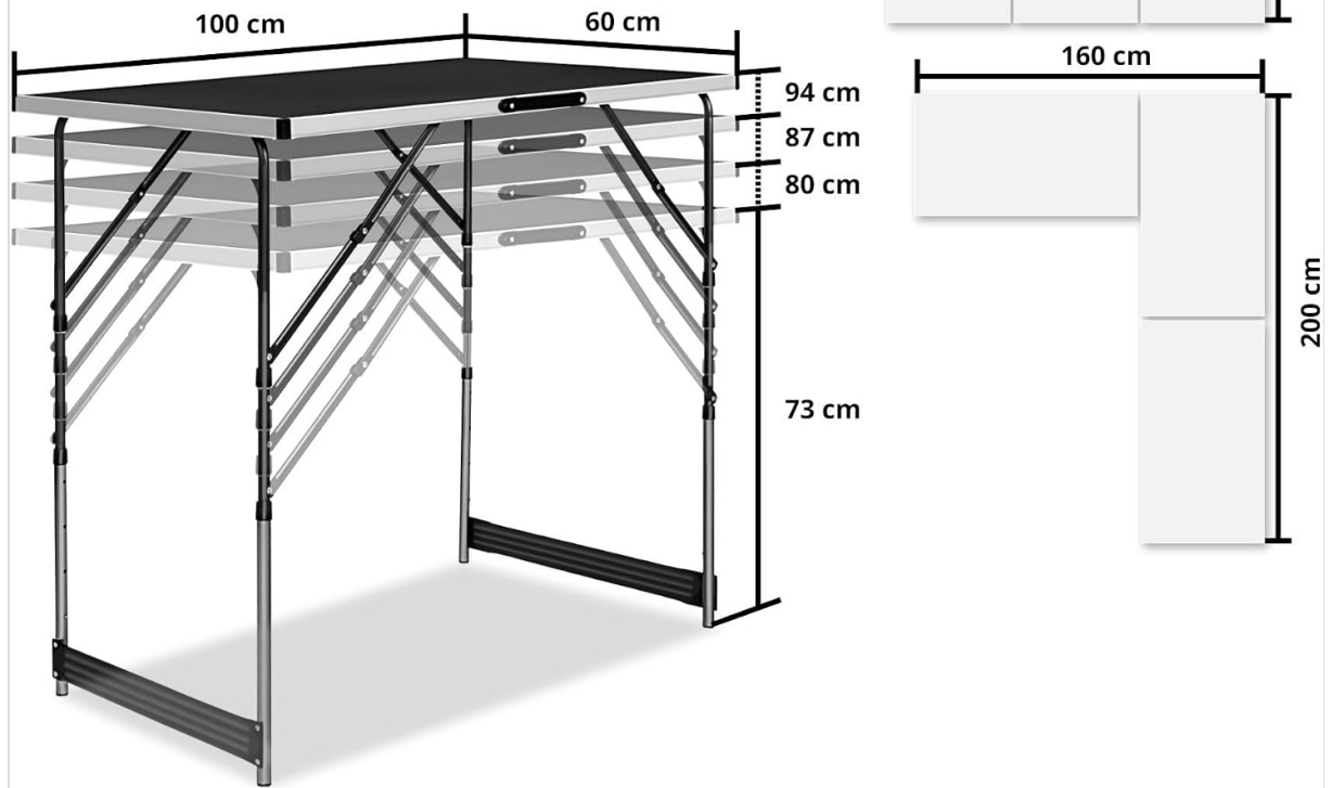
Figure 5: Detailed Product Measurements. This diagram provides precise dimensions for the table surface, weight, load capacity, and the four adjustable height settings.
