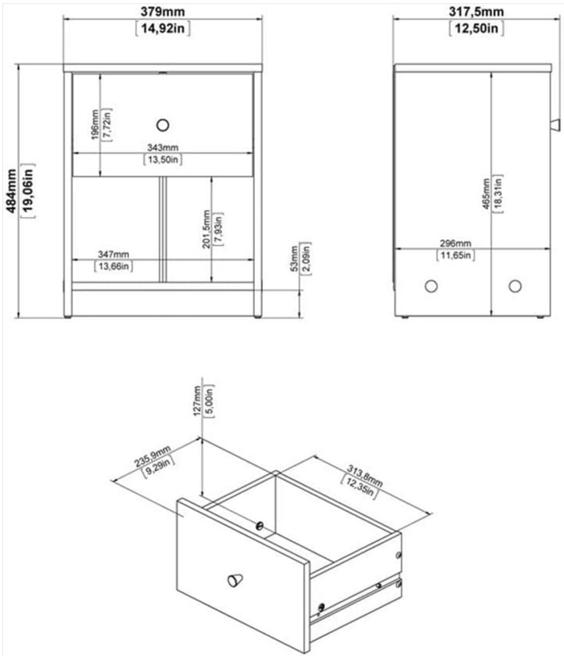
Image 4.1: Detailed dimensional drawing of the nightstand, including front and side views with measurements in millimeters and inches, and an exploded view of the drawer assembly.
