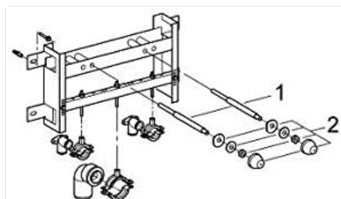
Figure 2: Exploded view of the Uniset Frame components. (1) Mounting rods, (2) Fixing plates/washers.
