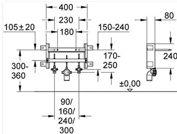
Figure 3: Technical drawing illustrating installation dimensions and variable distances for the Uniset Frame.
