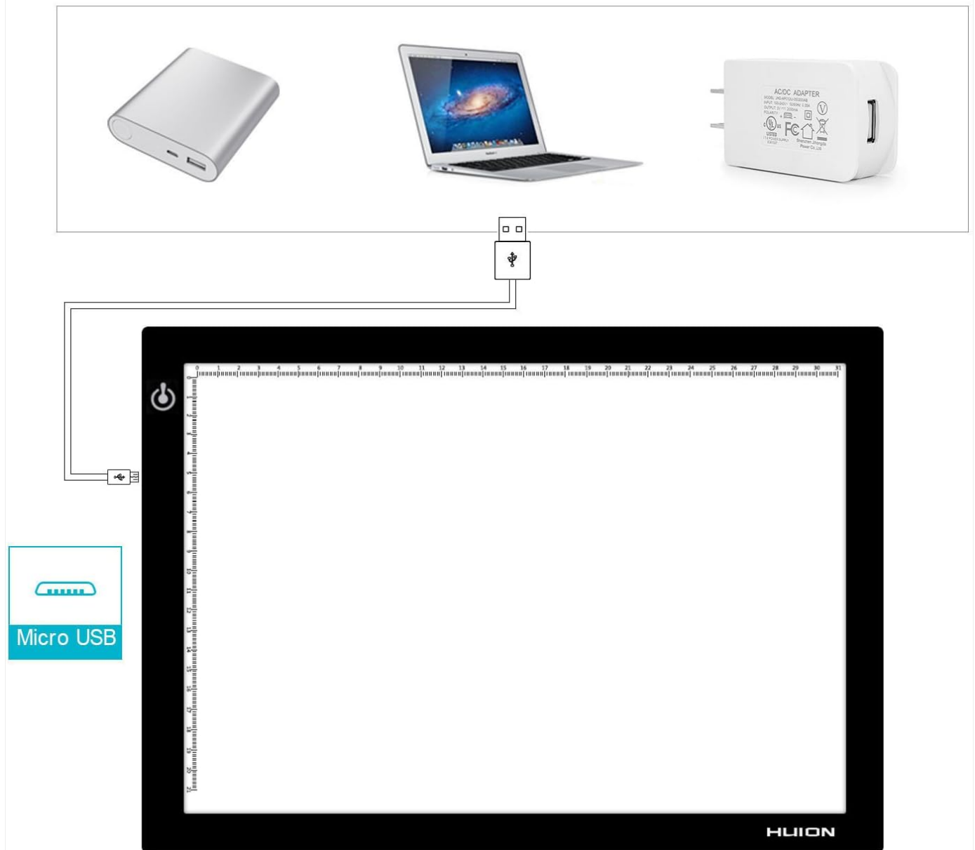
Figure 5: Powering the light box via USB from different sources.
