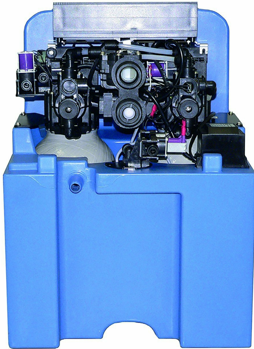
Figure 2: Internal view of the BWT AQA life S, showing key components for professional installation.
