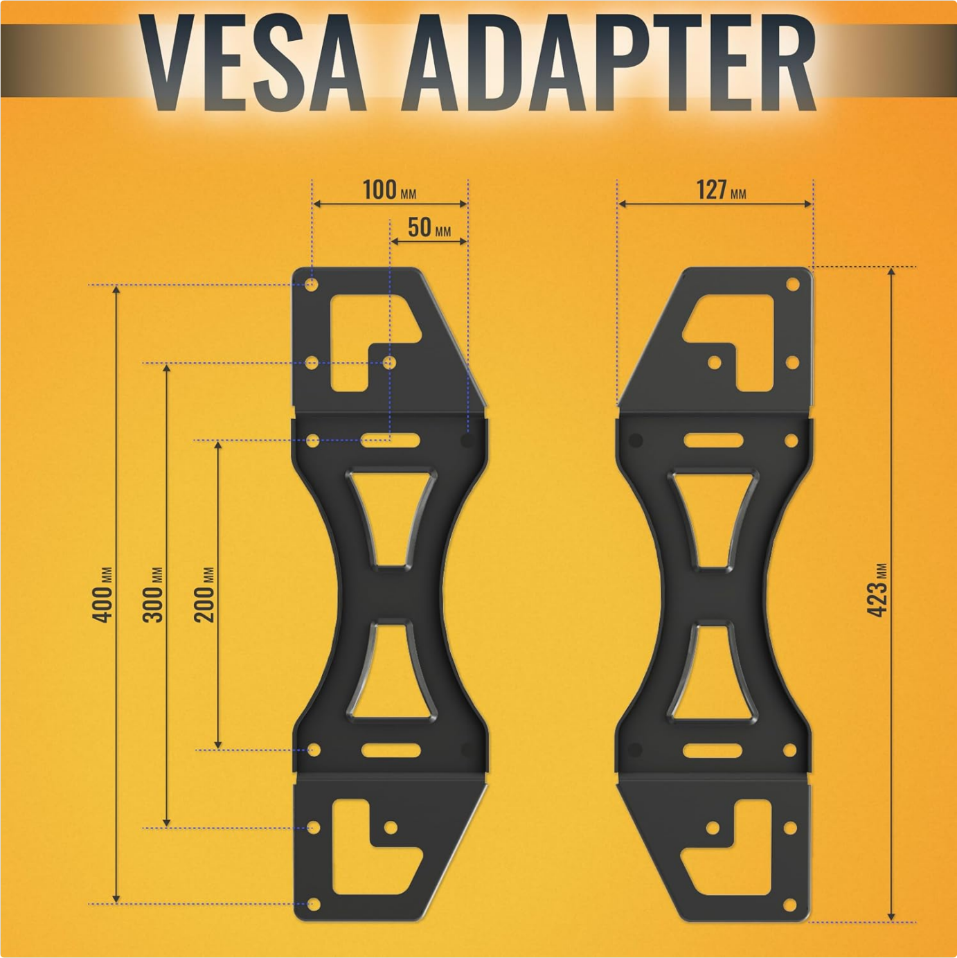
Image: Detailed dimensions of the RICOO VA0300 VESA adapter.
