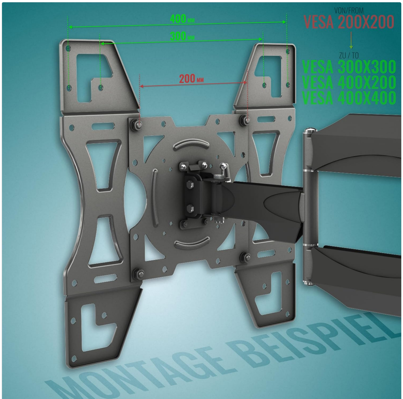
Image: Example of VESA 200x200 extended to 400x400 for TV mounting.
