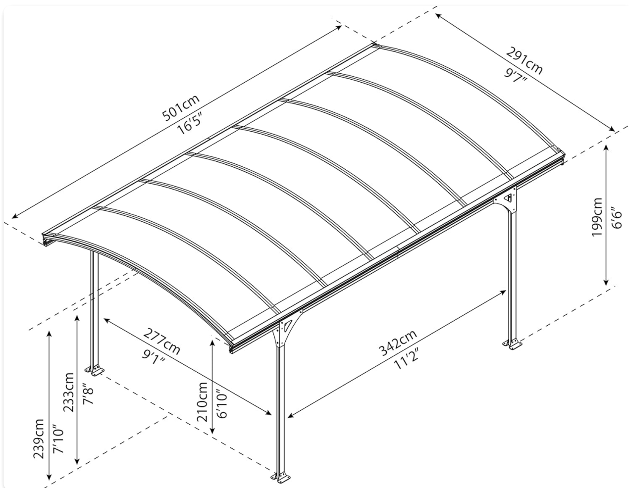
Image 3.3: Detailed diagram showing the overall dimensions of the Vitoria 5000 Carport.
