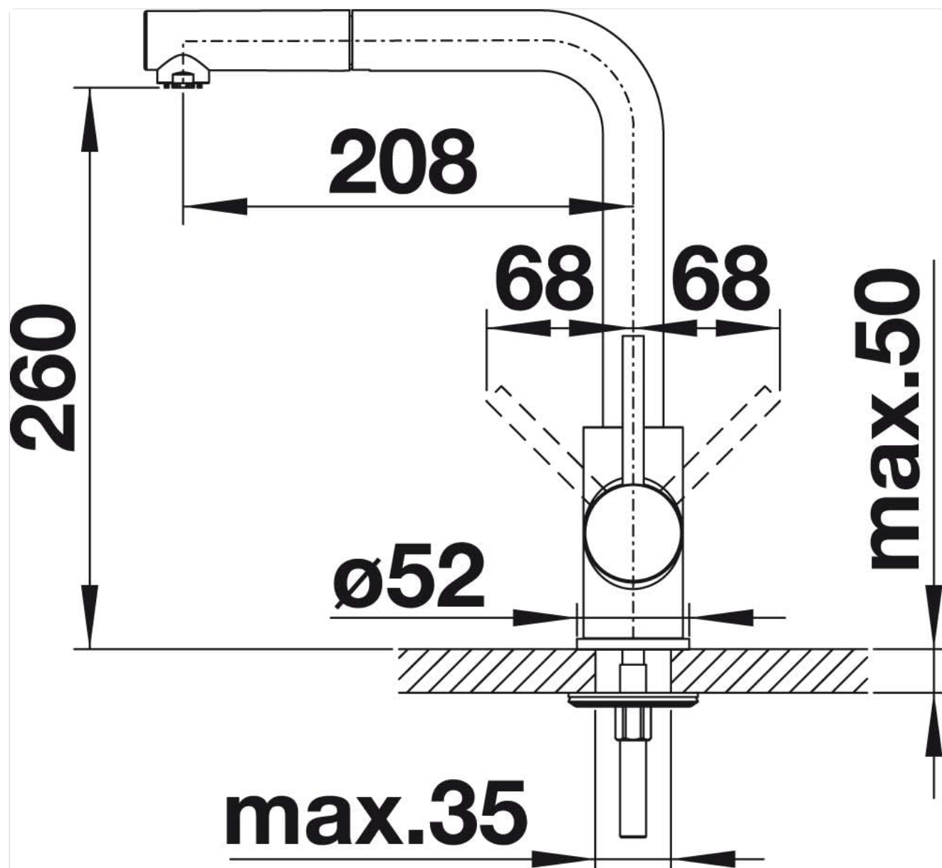
Figure 2: Front view dimensions of the BLANCO Mila-S faucet (measurements in mm).
