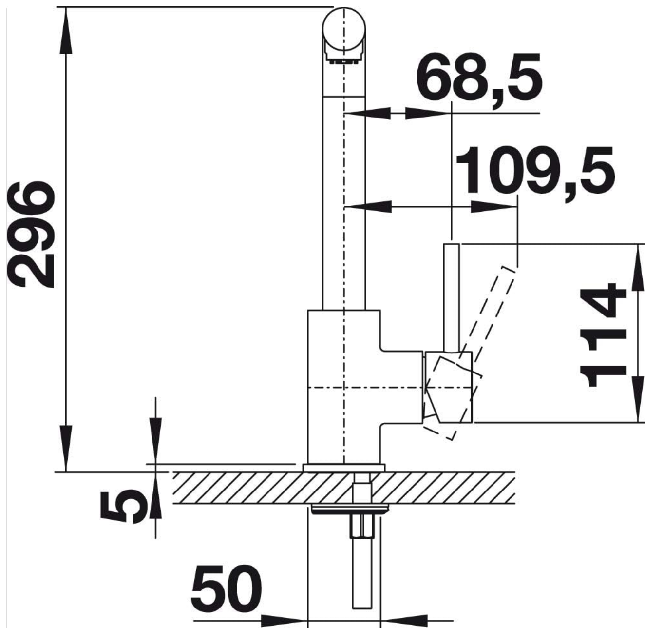
Figure 3: Side view dimensions of the BLANCO Mila-S faucet (measurements in mm).
