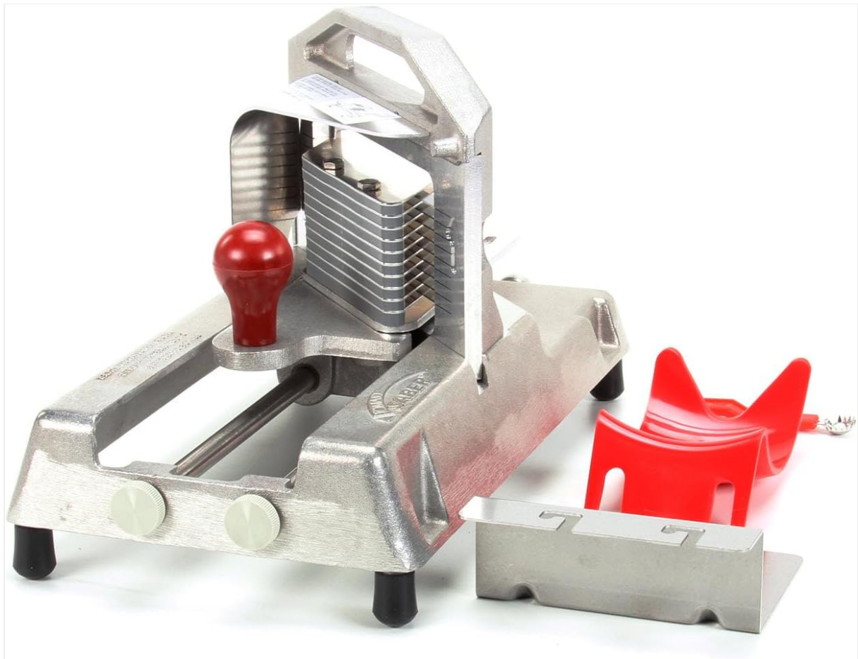
Figure 3: View of the slicer with the red push handle, ready for operation.
