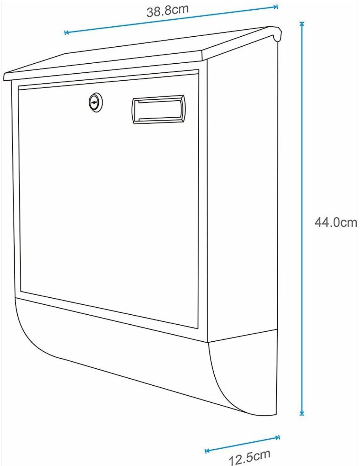
Image 2: Mailbox dimensions for installation planning. (Approx. 38.8 cm width, 44.0 cm height, 12.5 cm depth).
