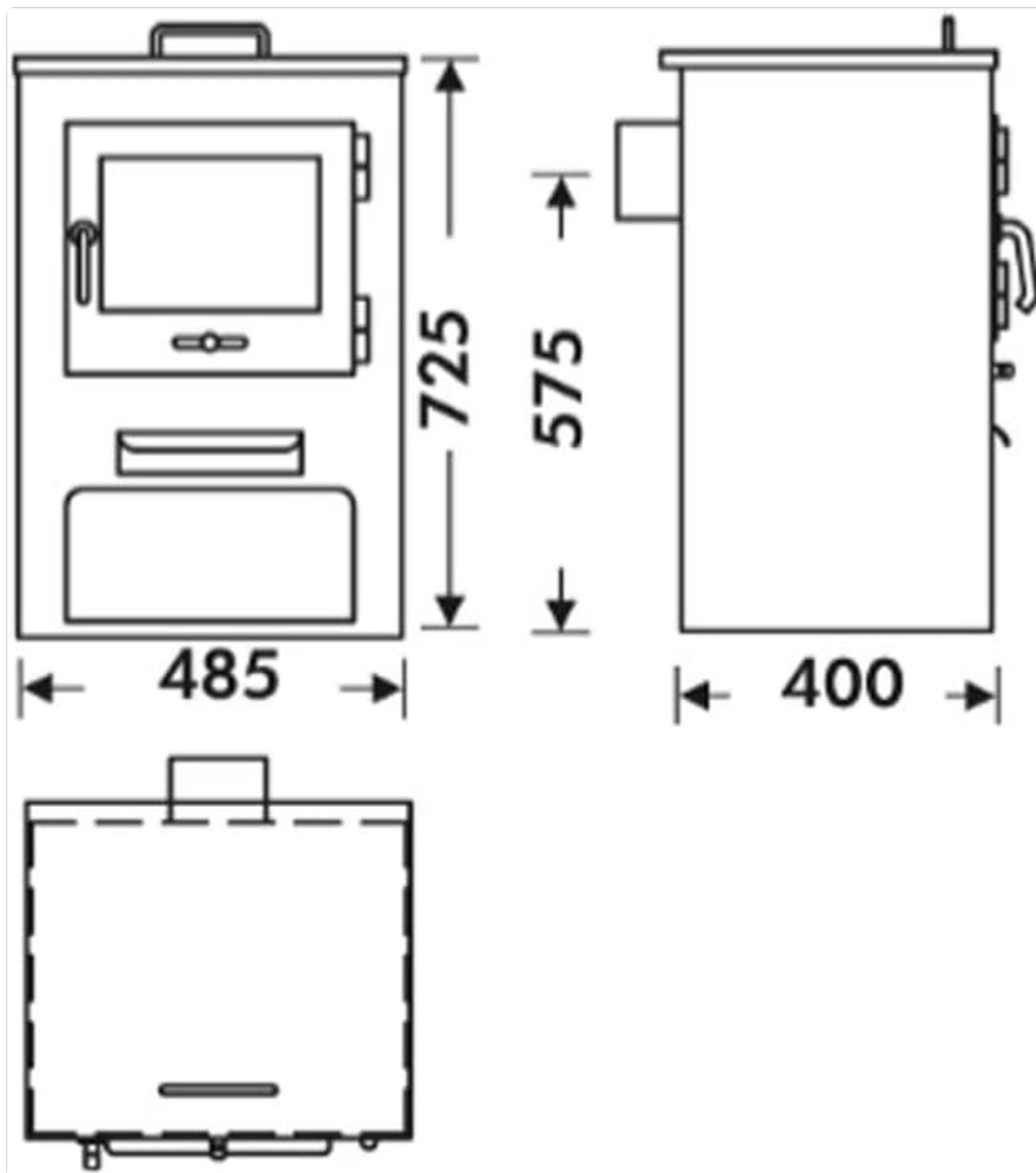
Image 4.1: Technical drawing with key dimensions of the Ibiza S Wood Stove.
