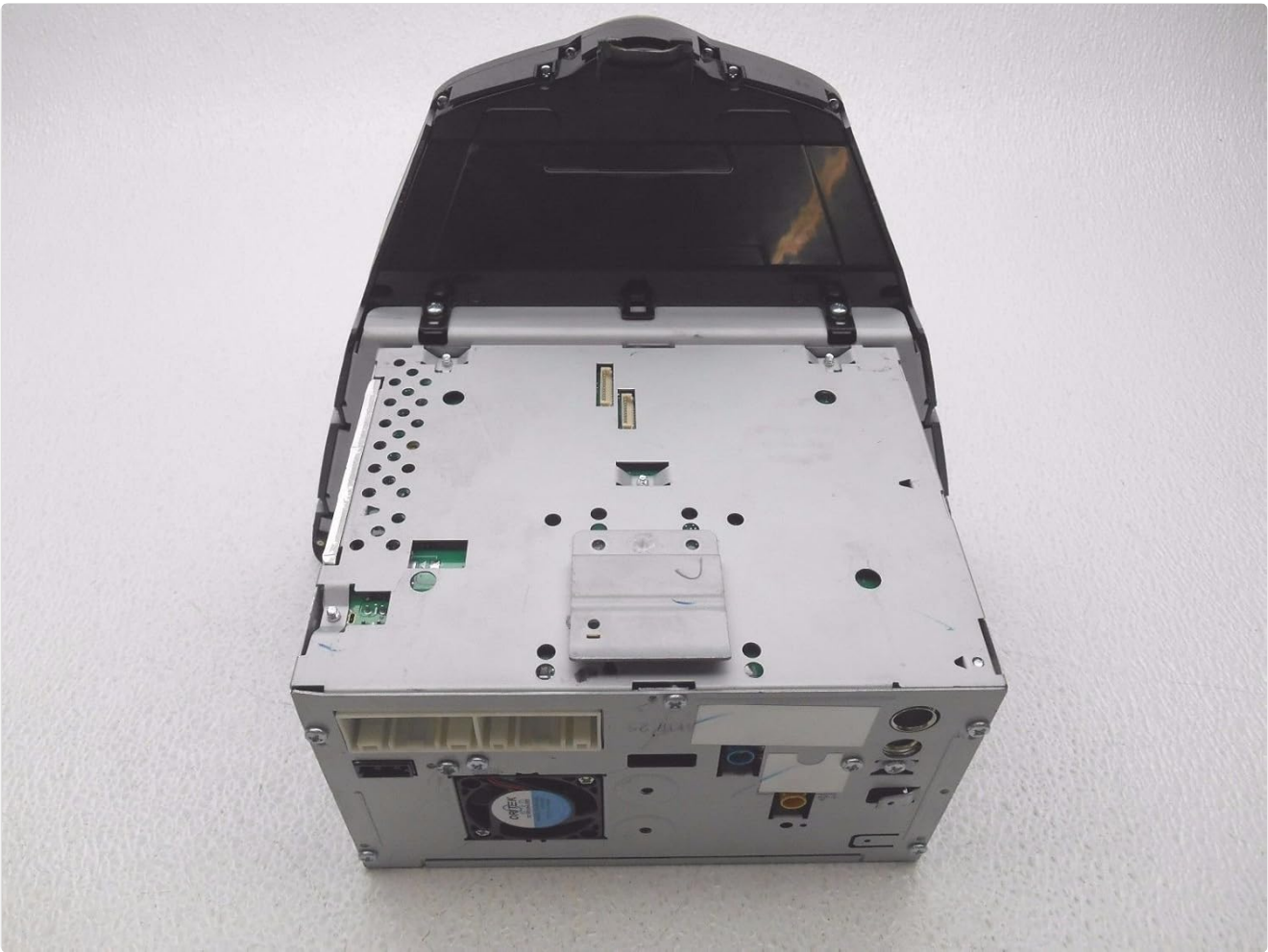
Figure 2.5: Top-down view of the head unit, showing the chassis and internal component housing.
