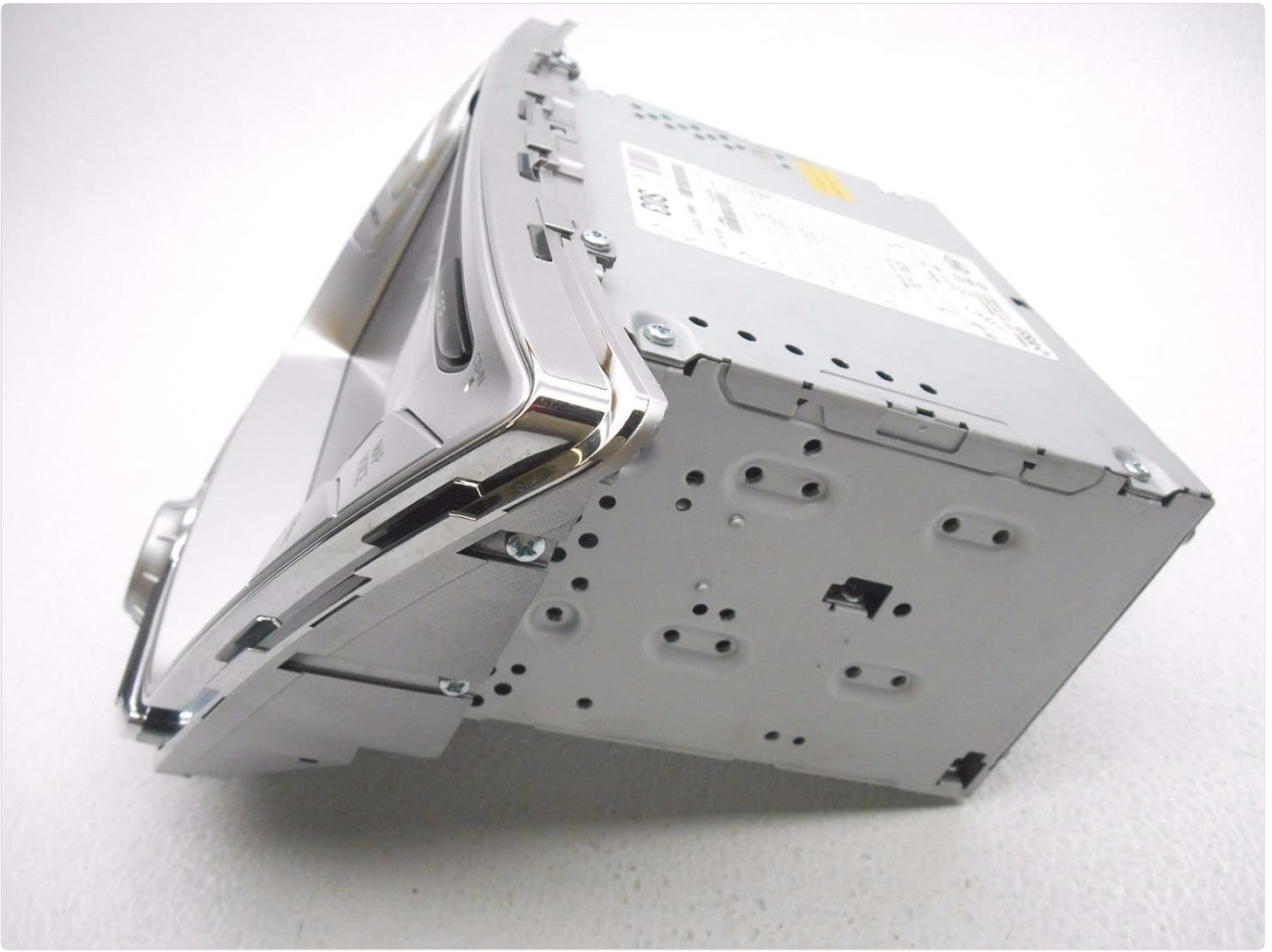
Figure 2.2: Side view of the head unit, illustrating its depth and typical mounting bracket attachment points.
